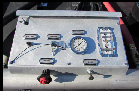
Top Mounted Controls
